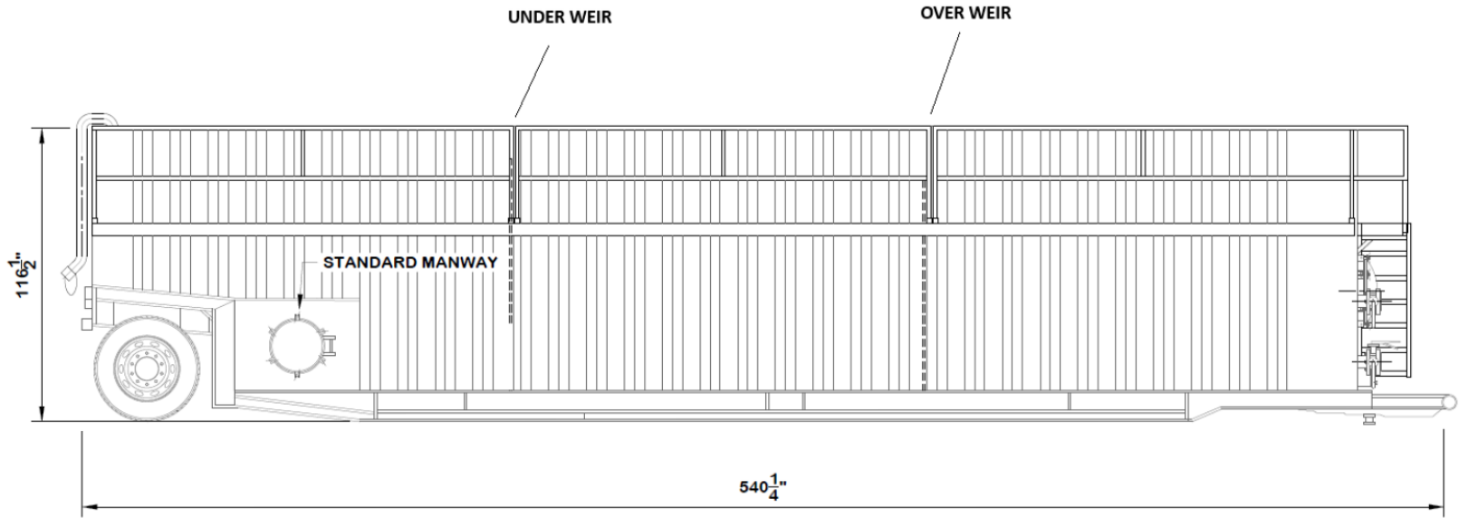
FRAC TANK - SIDE ELEVATION
